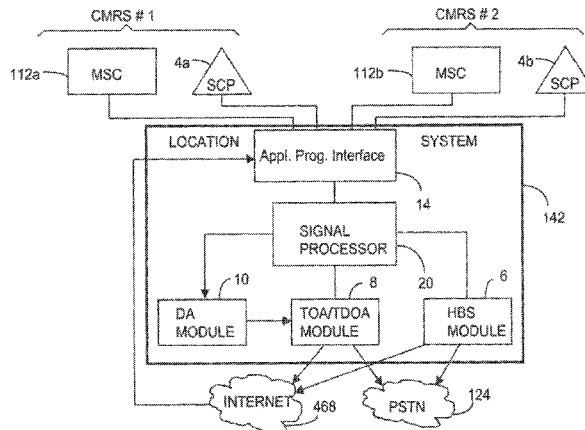
WIRELESS LOCATION USING MULTIPLE CMRSs
