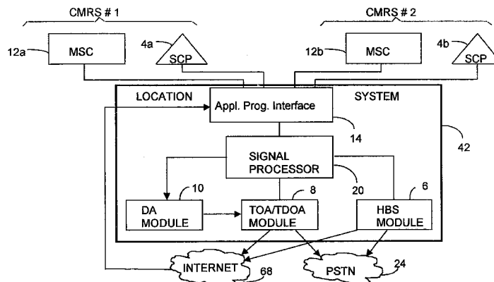
WIRELESS LOCATION USING MULTIPLE CMRRs
