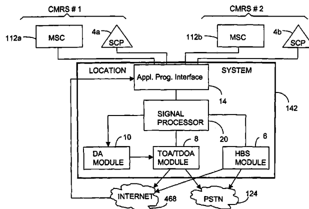
WIRELESS LOCATION USING MULTIPLE CMRSs
