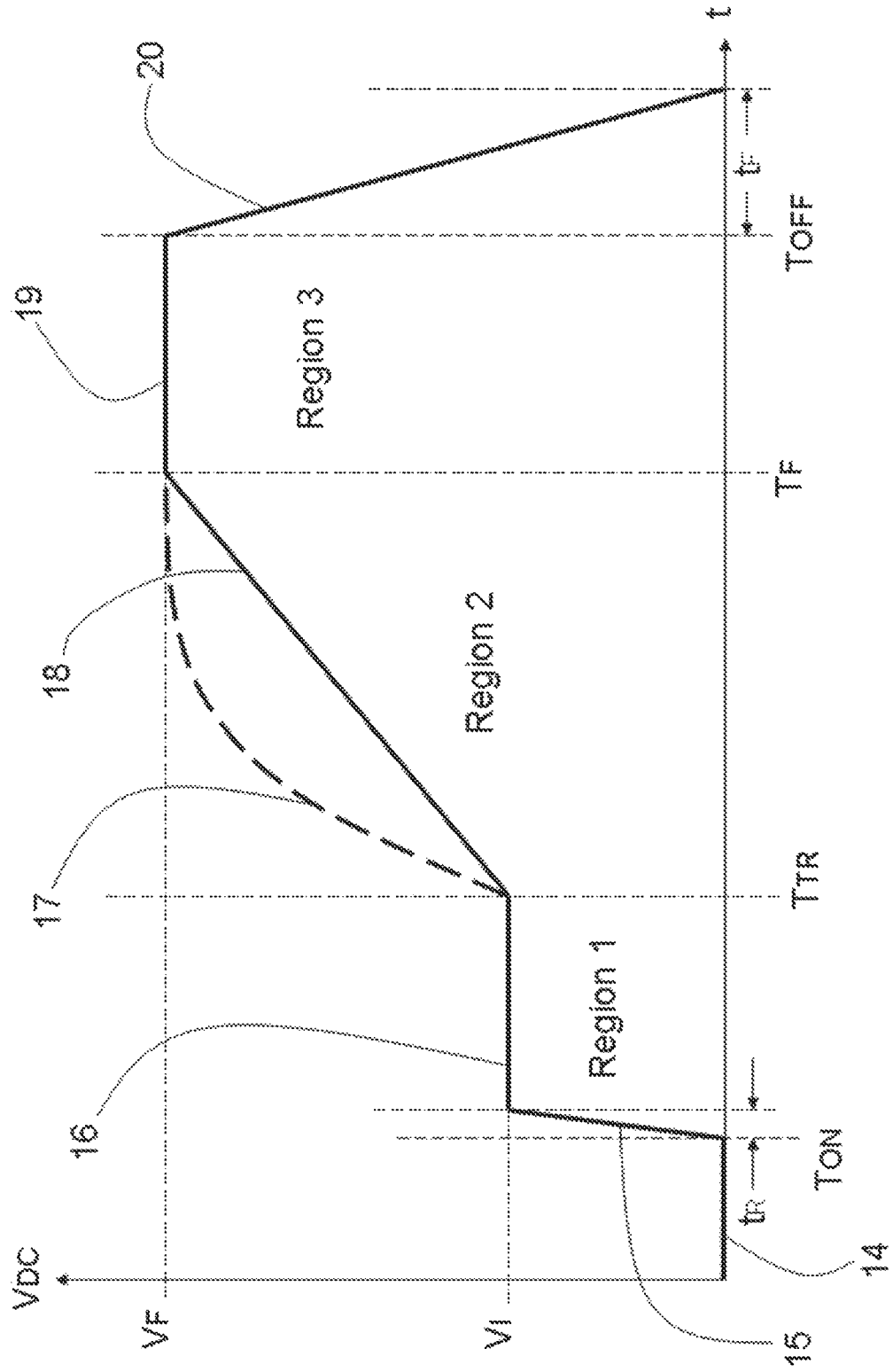
FIGURE 3. Enhanced Detector Bias
