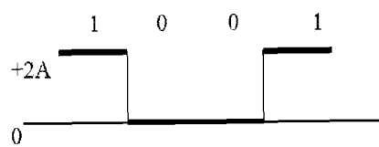
a) NRZ 1001 non-balanced pattern
